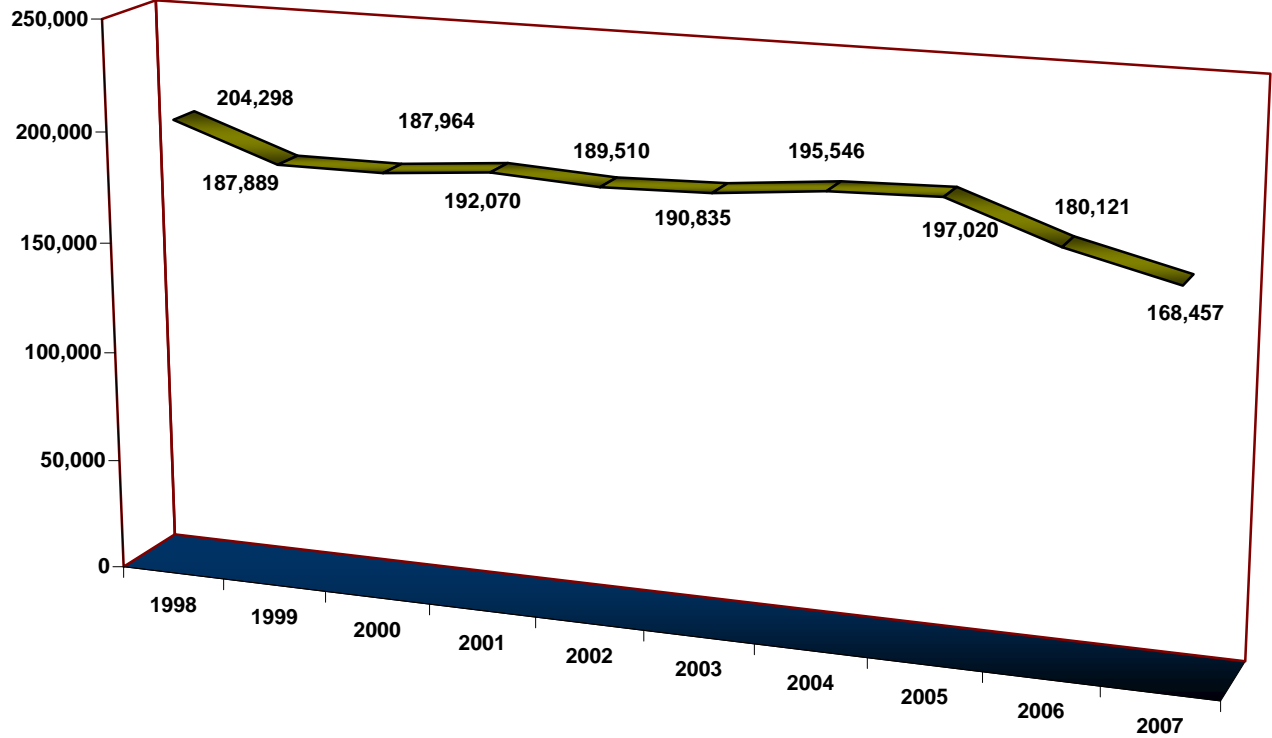
Larceny Theft 1998 - 2007
