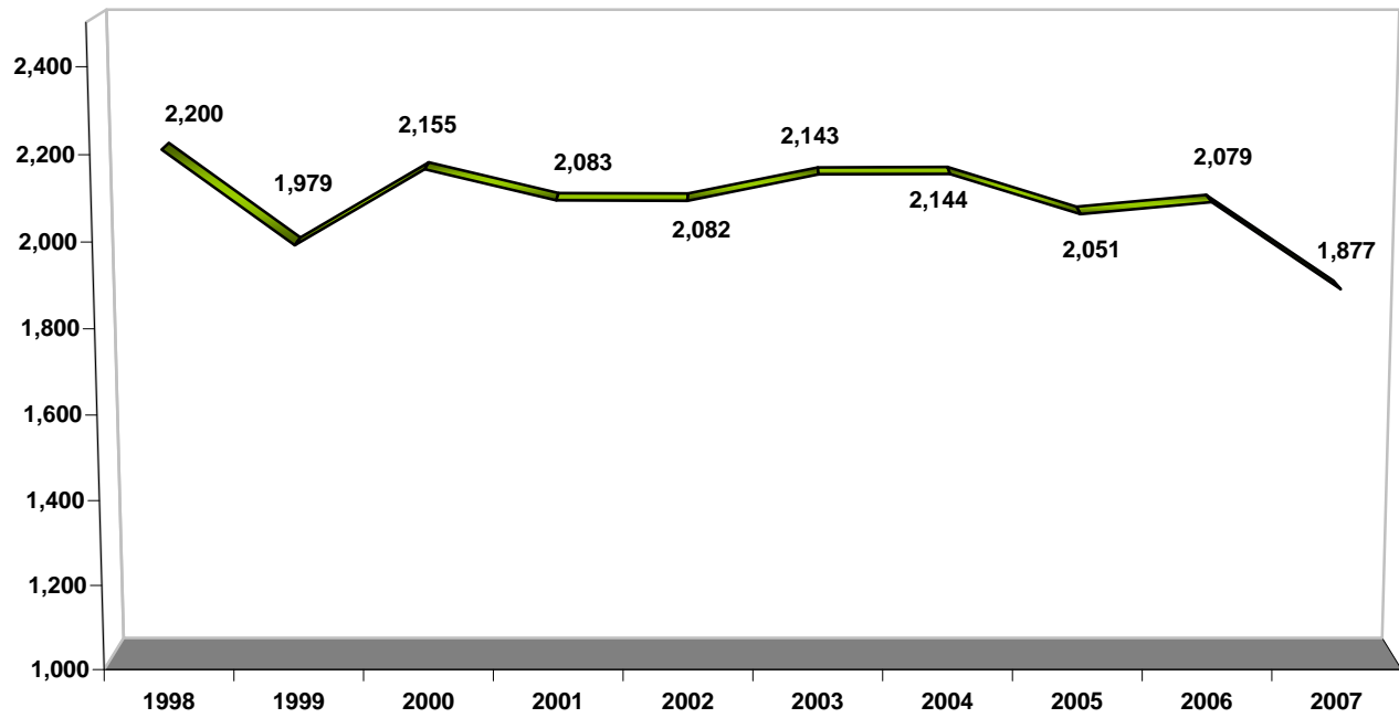
Arson Trend 1998 - 2007
